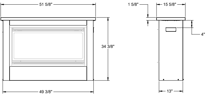
PL42VO ENCLOSURE
