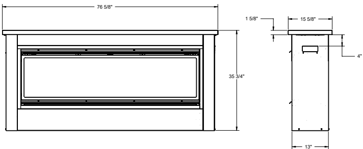
PL60VO ENCLOSURE
