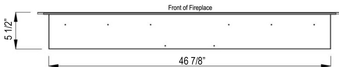
Top View
