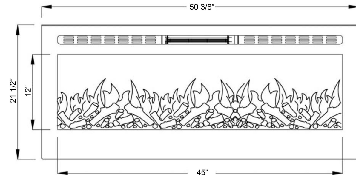
Front View
