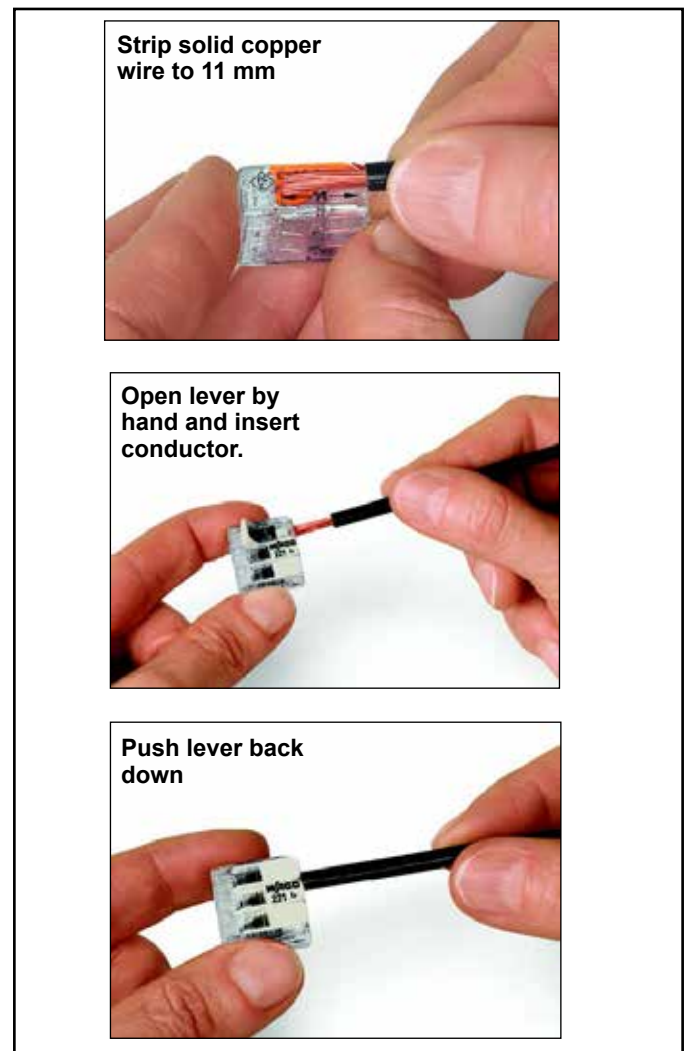
Figure 4.6 Wire Termination
