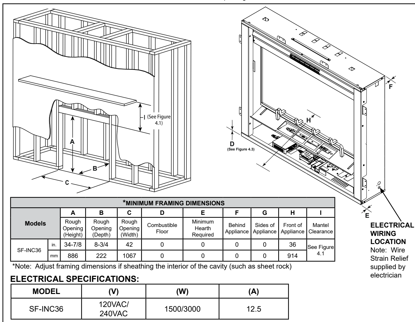
Figure 3.5 Framing Dimension
