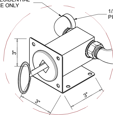
BRACKET DETAIL
