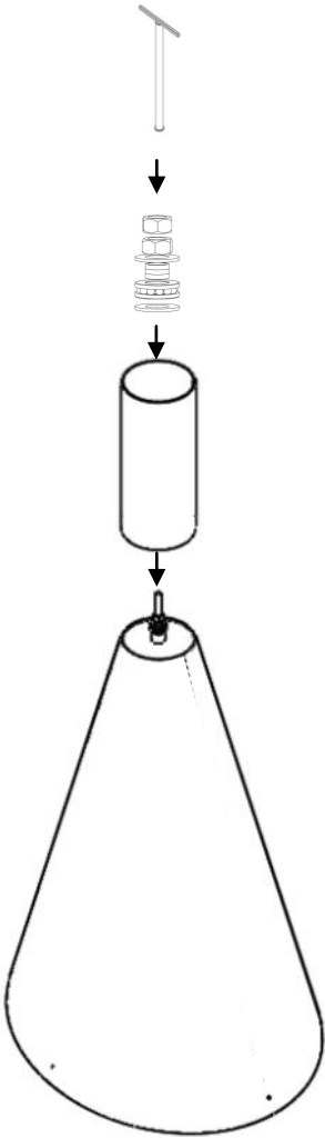
Figure 4— Assembly representation
