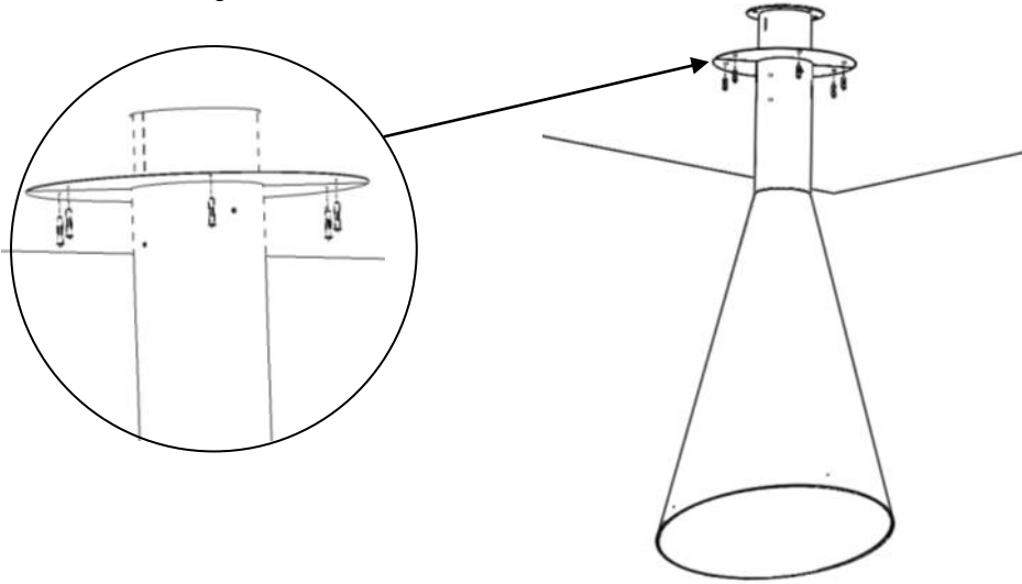
Figure 7 — Ceiling finishing mirrors
