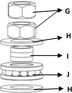
Figura 3— Assembly order
