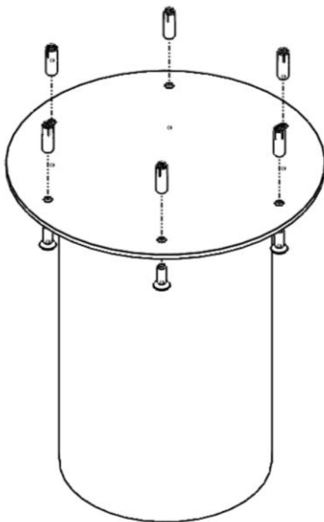
Figure 1 – Top part to screw to the ceiling
