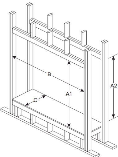
Floor Install
