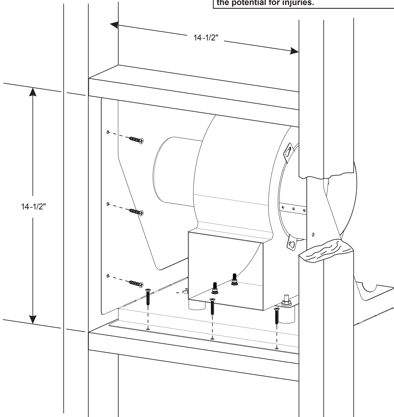
HMFA Framing Install Figure 3
