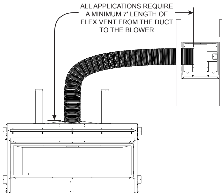
Minimum Length Of Flex Vent
