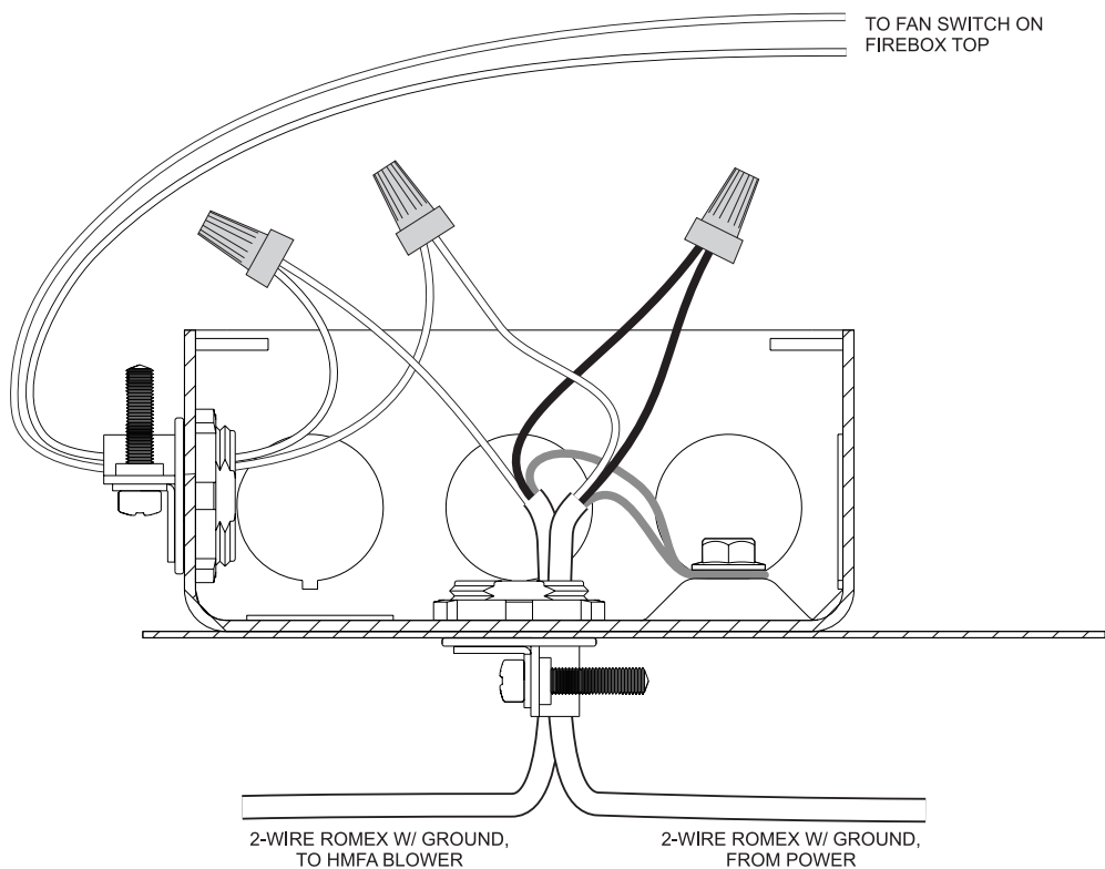
Connect Fan Switch To Power
